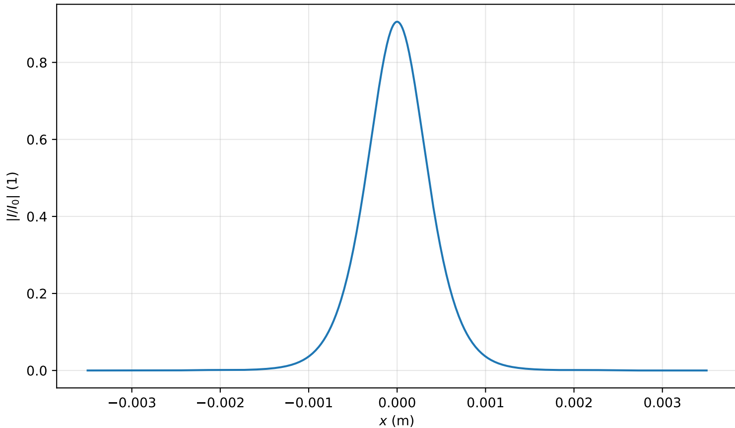
Intensity profile I(x, y = 0, z = 3.821m)/I_0 , P_{in}=0.8P_{cr} , artificial time
